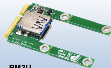
PM3U (MiniCard to USB2.0 adapter) x1
