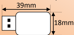
MiniCard slot (Full Size) Max USB device body size:
